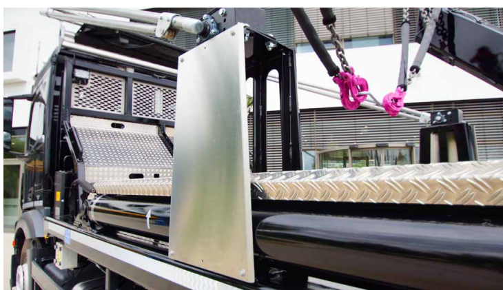
Fixation of the system on the superstructure
